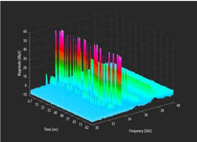
Fig. 7 – Real-time measurement of a GHz frequency hopping signal.
